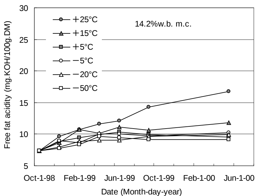
Figure 4 - Changes in free fat acidity of rice of 14.2% m.c. stored at six temperature levels.
