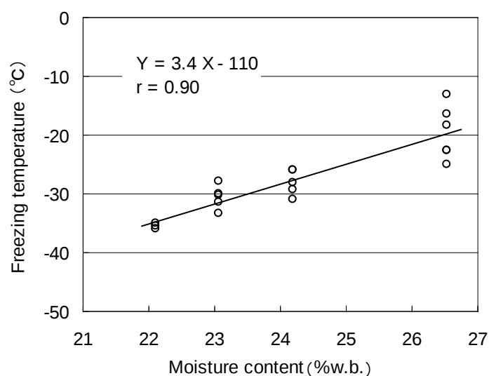
Figure 1 - Relationship between moisture content and freezing temperature of rice.
