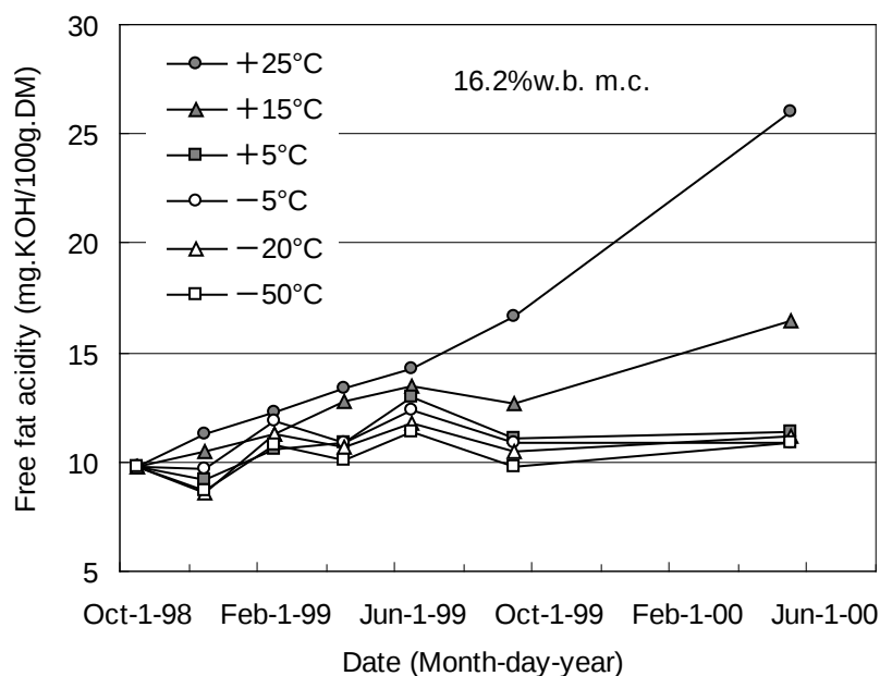
Figure 3 - Changes in free fat acidity of rice of 16.2% m.c. stored at six temperature levels.
